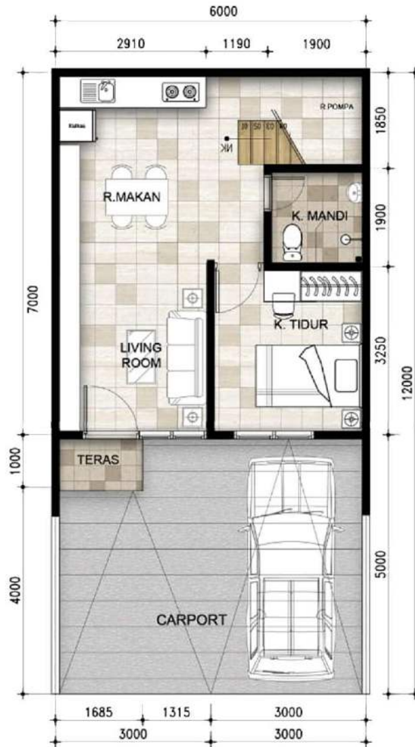
DENAH LANTAI 1
